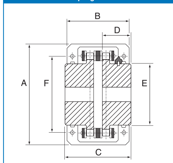
Chain Coupling Dimensions
